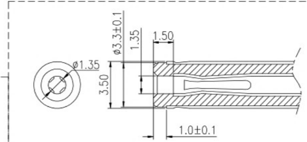
MATE PLUG
